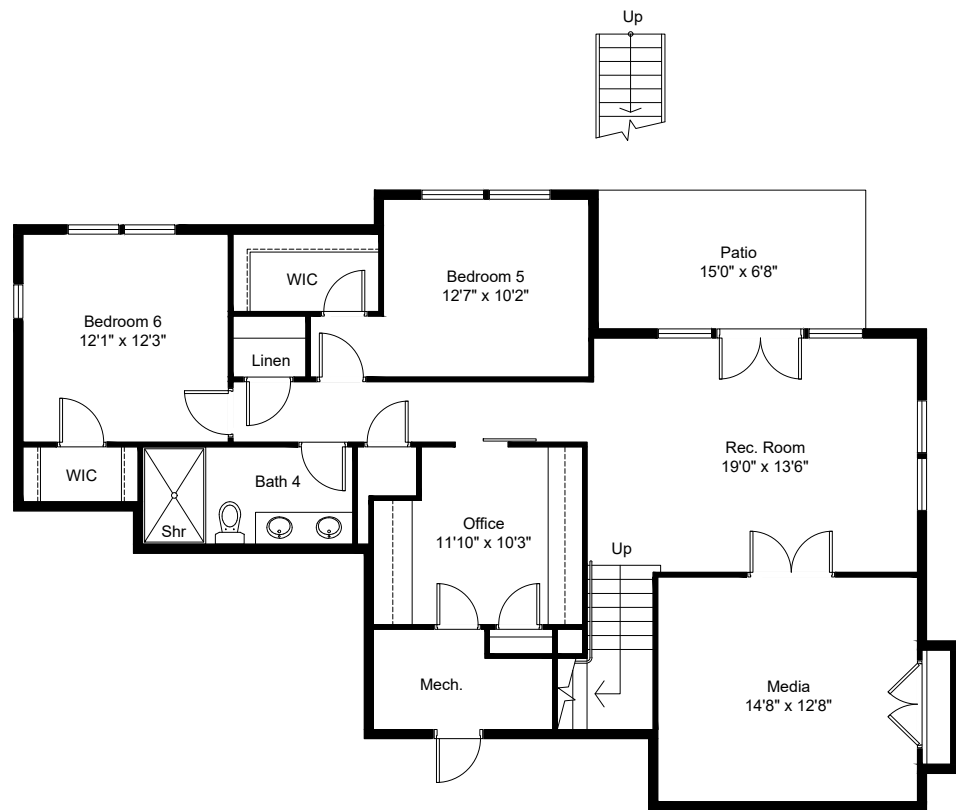
BASEMENT PLAN
